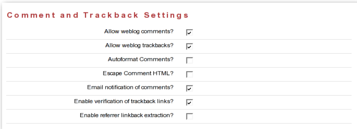
Illustration 27: Config: comments
